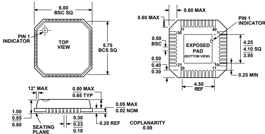
Figure 43. 40-Lead Lead Frame Chip Scale Package [LFCSP_VQ] 6 mm x 6 mm Body, Very Thin Quad (CP-40)
