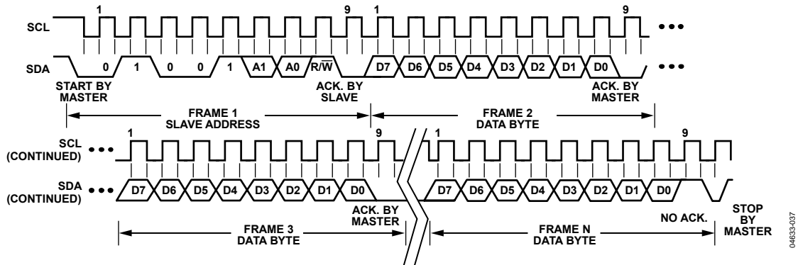
Figure 32. General SMBus Read Timing Diagram
